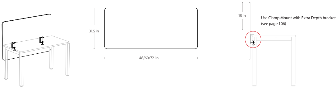
Axis Desk Hung Screens
