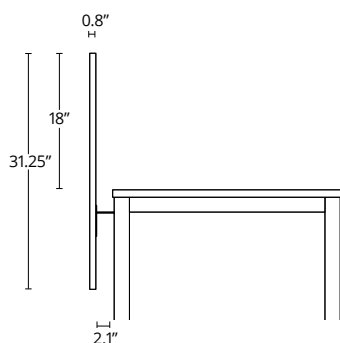
Offset Bracket
