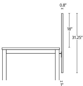
Standard Bracket
